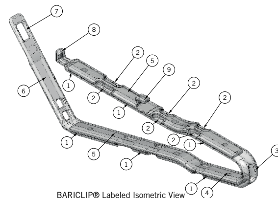
BARICLIP® Labeled Isometric View
